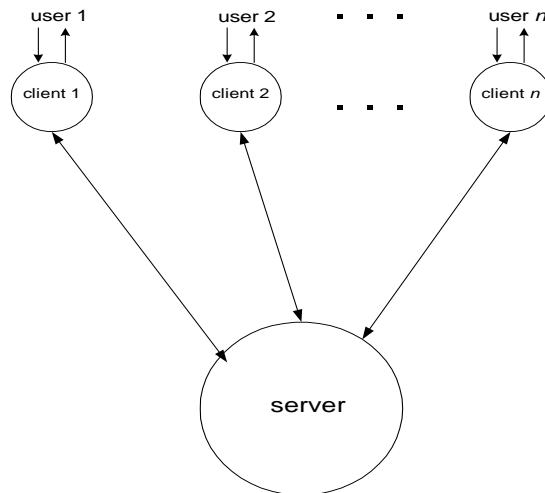
Gambar client-server architecture
